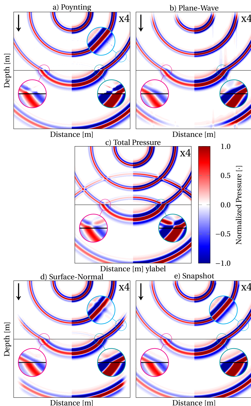
Figure 3.1: Comparison of different wavefield decomposition techniques applicable to RTM for the down-going wavefield. The right-hand-side amplitudes of each figure are exaggerated by a factor of four.
