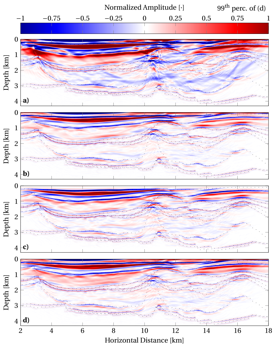
Figure 5.8: Comparison of stacked smoothed Annrveen migration results using conventional RTM (a), Poynting RTM (b), analytic RTM (c), and snapshot decomposition (d). Amplitudes have been normalized to the 99 th percentile of (d).
